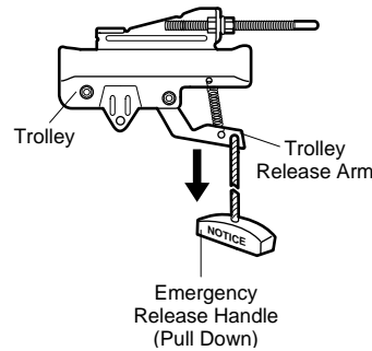
Manual disconnect position
