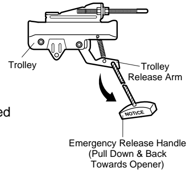
Lockout position
