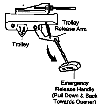
Lockout position
