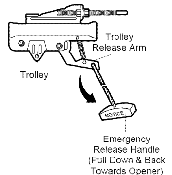
Lockout position
