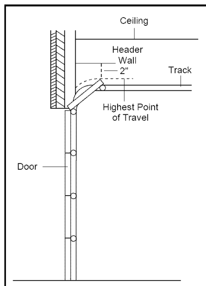
Sectional door with curved track
