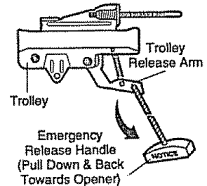
Lockout position
