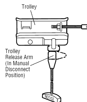
Lockout position (Manual disconnect)
