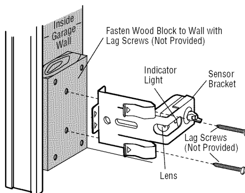
Figure 2 WALL MOUNT (RIGHT SIDE)
