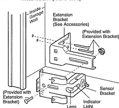
Figure 3 WALL MOUNT (RIGHT SIDE)
