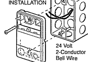
Figure 2 PRE-WIRED INSTALLATION
