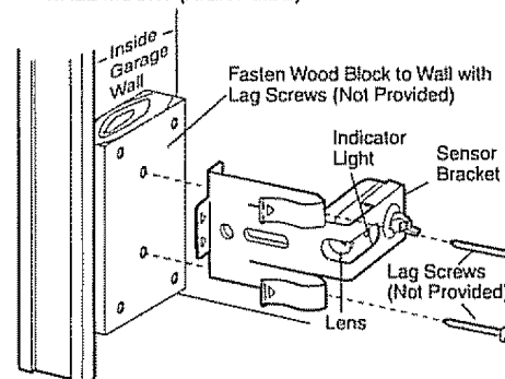
Figure 3 WALL MOUNT (RIGHT SIDE)
