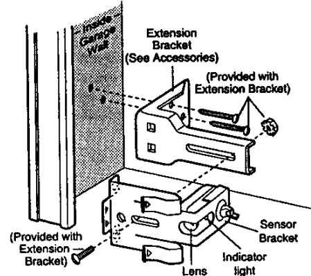
Figure 2 WALL MOUNT (Right Side)
