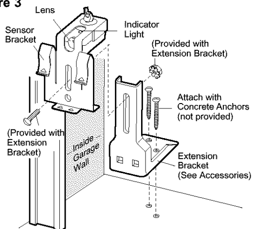
FLOOR MOUNT (RIGHT SIDE)
