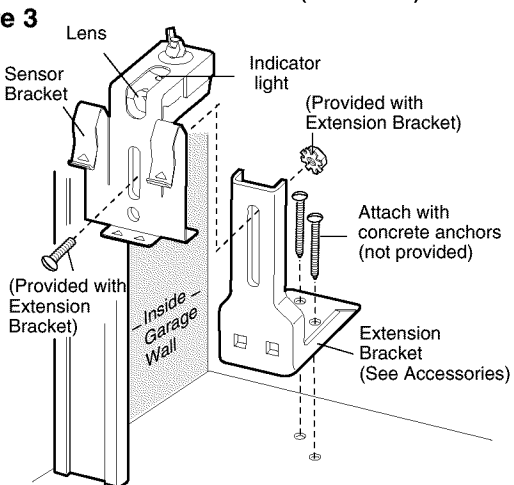
FLOOR MOUNT (RIGHT SIDE)
