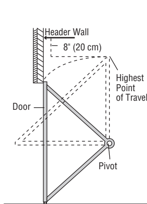
One-piece door without track: pivot hardware
