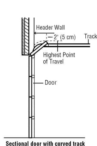
Sectional door with curved track
