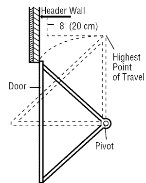
One-piece door without track: pivot hardware
